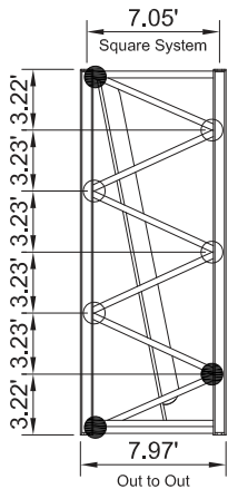
TYPICAL TS 212 TOWER SECTION ONLY (ELEVATIONS)
