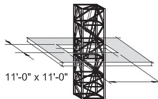
SLAB OPENING Recommended for TS212
